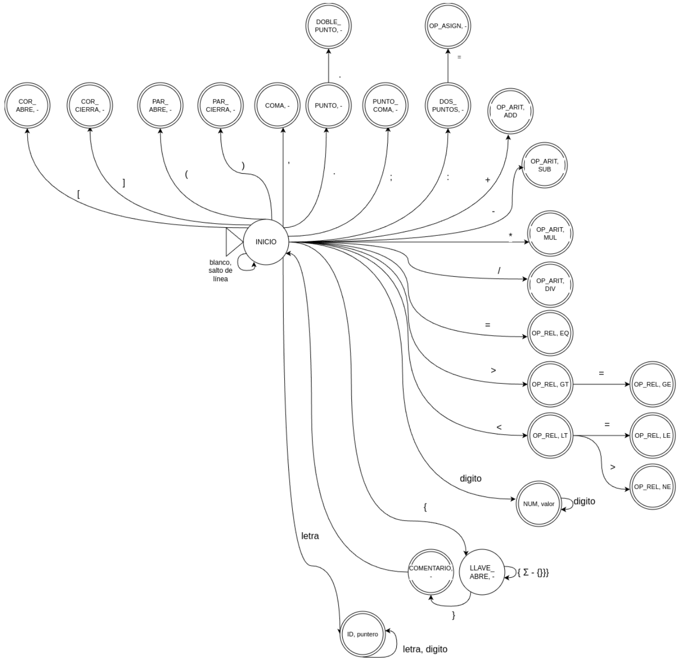
Figure 1: Autómata Finito
